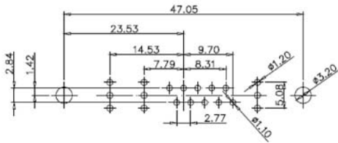
13W6 Male
