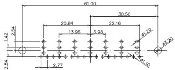
24W7 Male/Female
