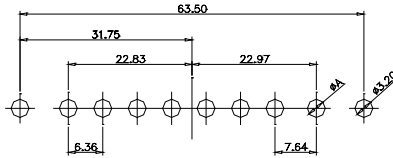
CODE:8W8 FEMALE
