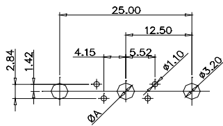
CODE:7W2 MALE/FEMALE
