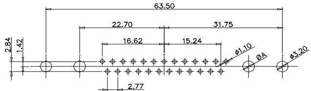
CODE:21W1 MALE/FEMALE
