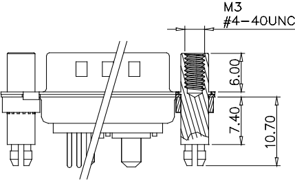
CODE:6/E
