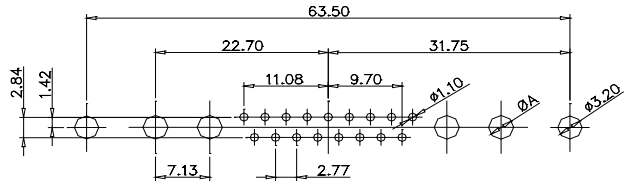
CODE:27W2 MALE/FEMALE
