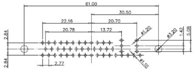
43W2 Male
