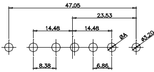
CODE:5W5 FEMALE
