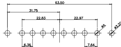
CODE:8W8 FEMALE
