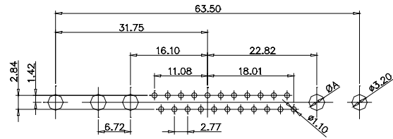
CODE:36W4 MALE
