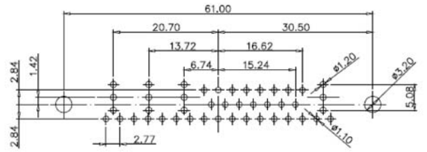
36W4 Male
