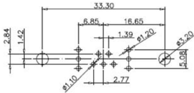
11W1 Male/Female
