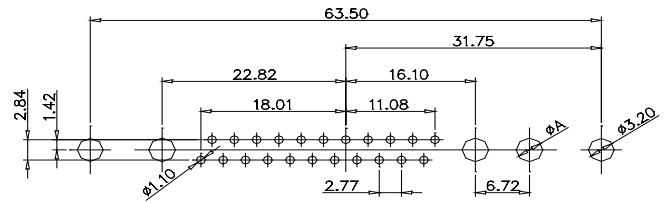
CODE:36W4 FEMALE
