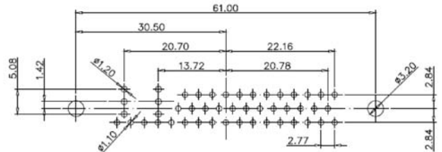
43W2 Female
