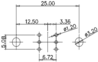
CODE:2W2/2WK2
