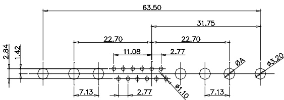
CODE:17W5 MALE
